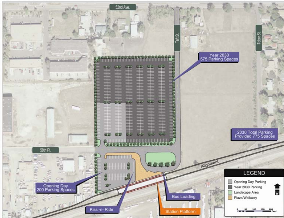
FIGURE 2-29 Ward Road Station (2015 and 2030, all surface parking)
