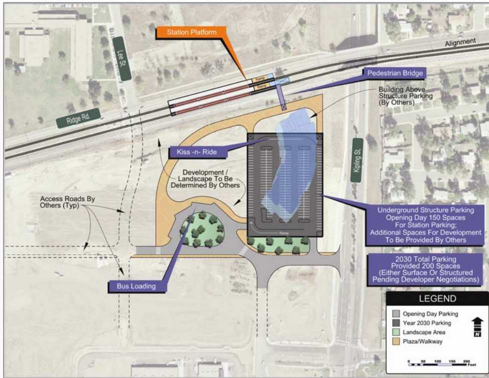
FIGURE 2-28 Arvada Ridge Station (2015 and 2030, parking may be surface or structured pending developer involvement)
